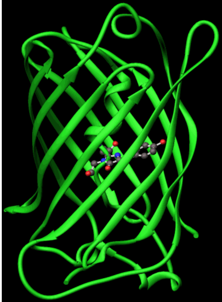
Figure 2. Ribbon diagram of the Green Fluorescent Protein (GFP) drawn from the wild-type crystal structure. The buried chromophore, which is responsible for GFP's luminescence, is shown in full atomic detail.
